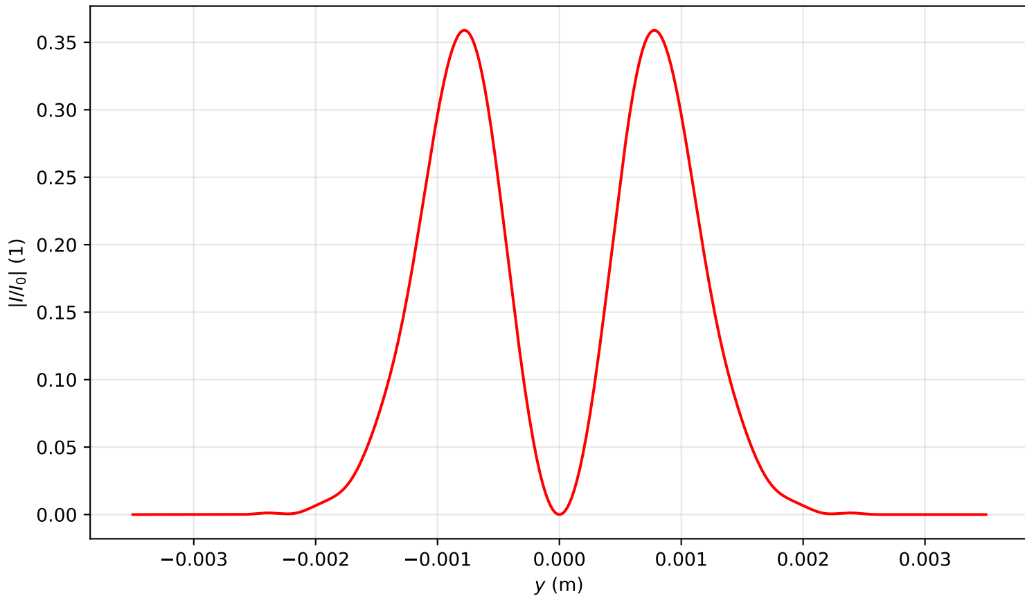
Intensity profile I(x=0, y, z=2.786)/I_0 , \text{Pin}=2.0\text{Pcr} , artificial time
